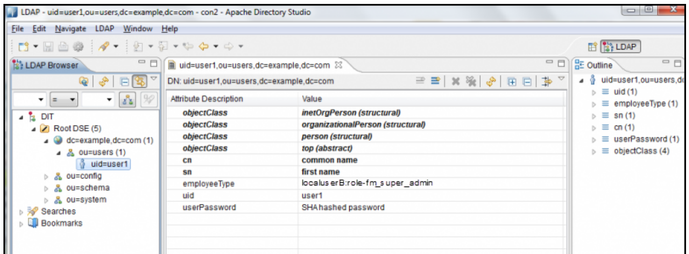
Figure 15 Adding the employeeType Attribute
