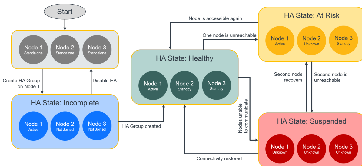
Figure 43 High Availability States
