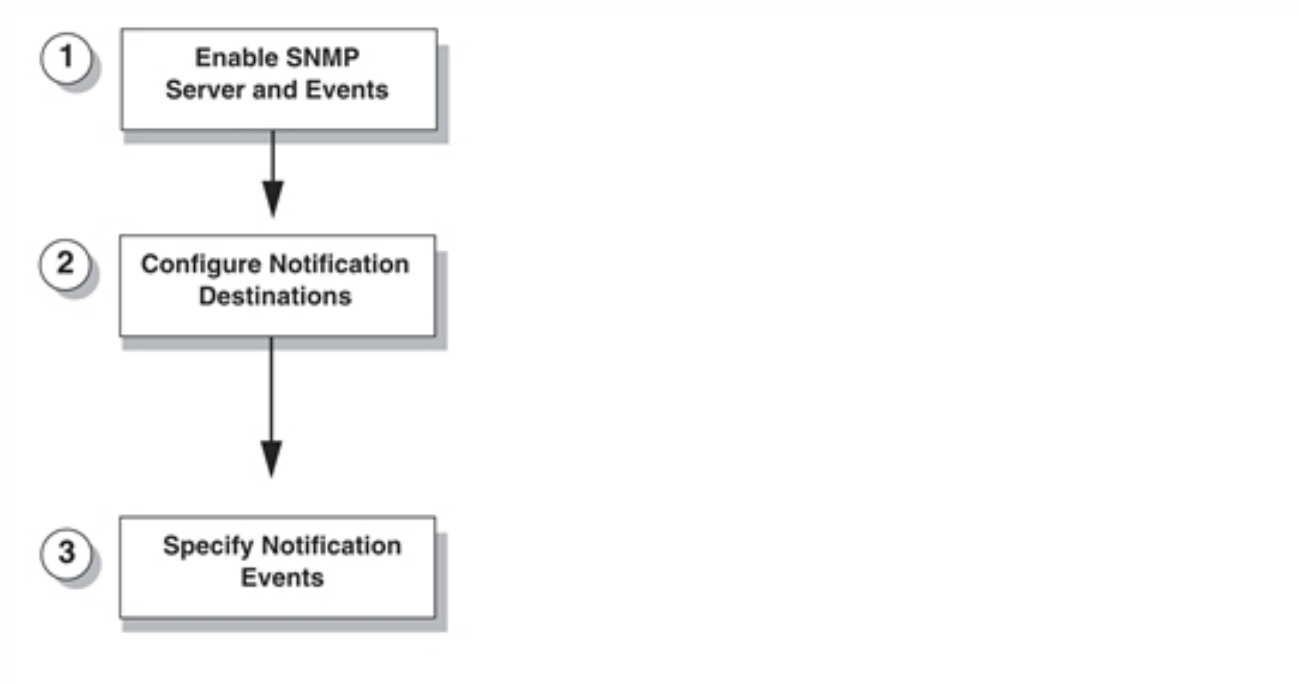
Figure 36 Configuring SNMP Notifications
