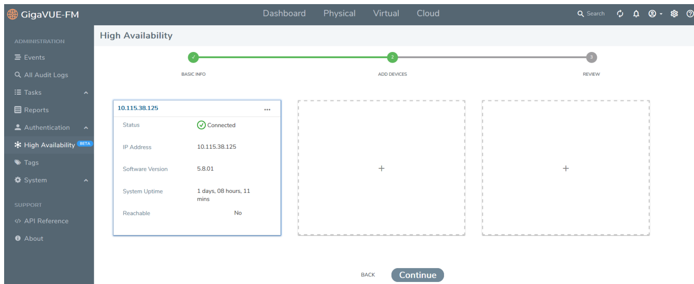
Figure 40 Add GigaVUE-FM Instances to the HA Group
