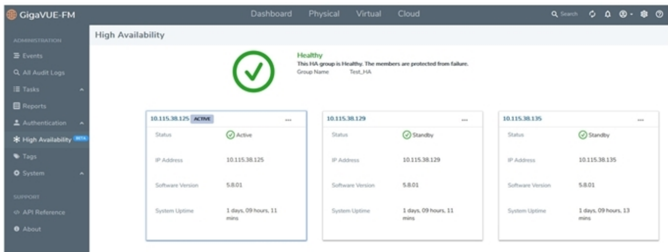
Figure 41 GigaVUE-FM HA Group Created
