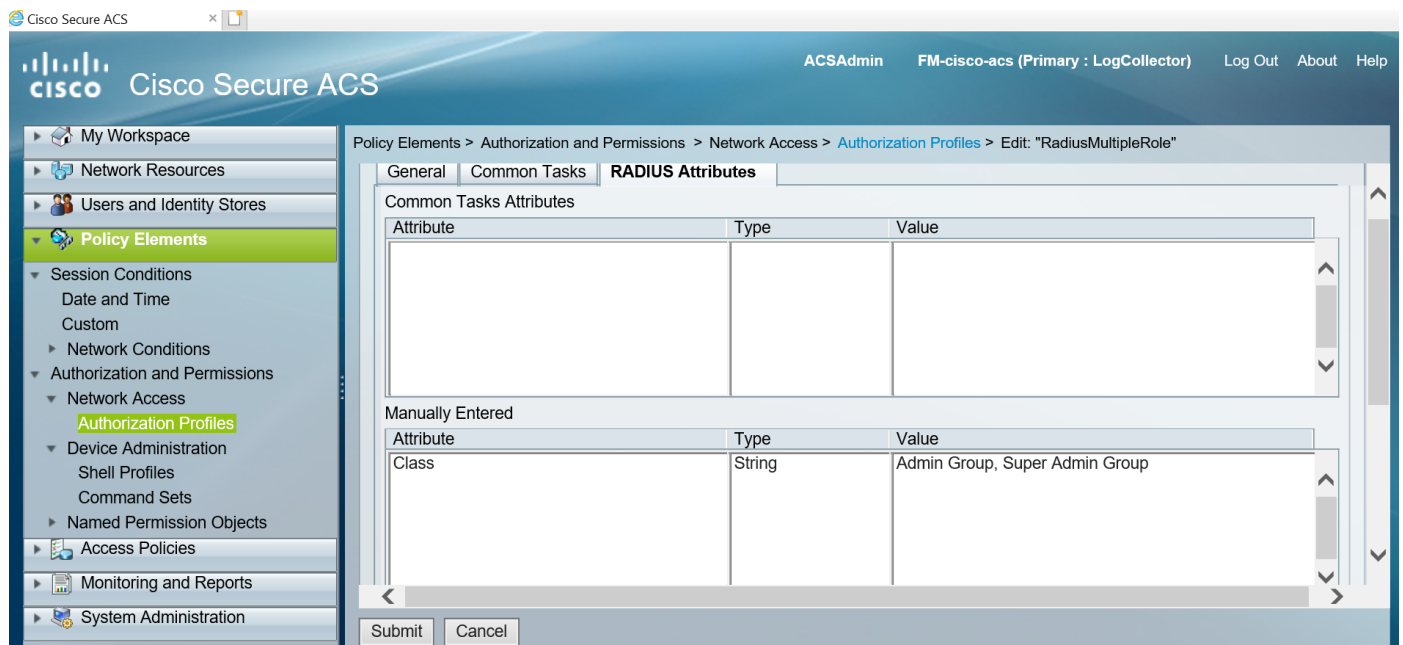
Figure 6 Supplying the Class Field for RADIUS (ACS 5.x)
